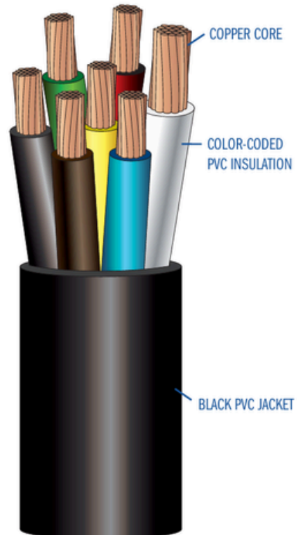
INSULATED 7-WIRE
